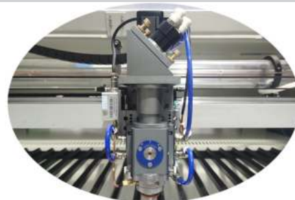
Mixed cutting laser head
